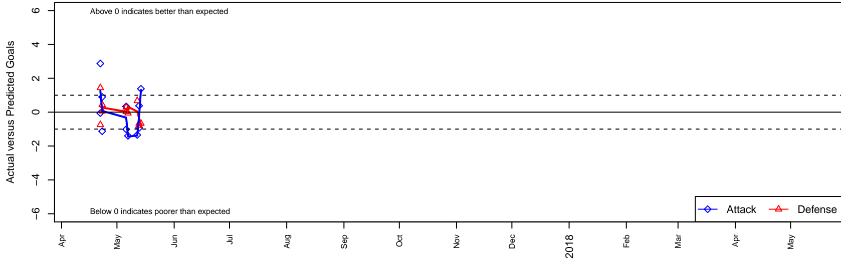
BYSL Bluebirdz B04 Dots are actual minus expected GF (blue circles) and GA (red triangles). Blue line is smoothed change in attack strength. Red is smoothed change in defense strength.
